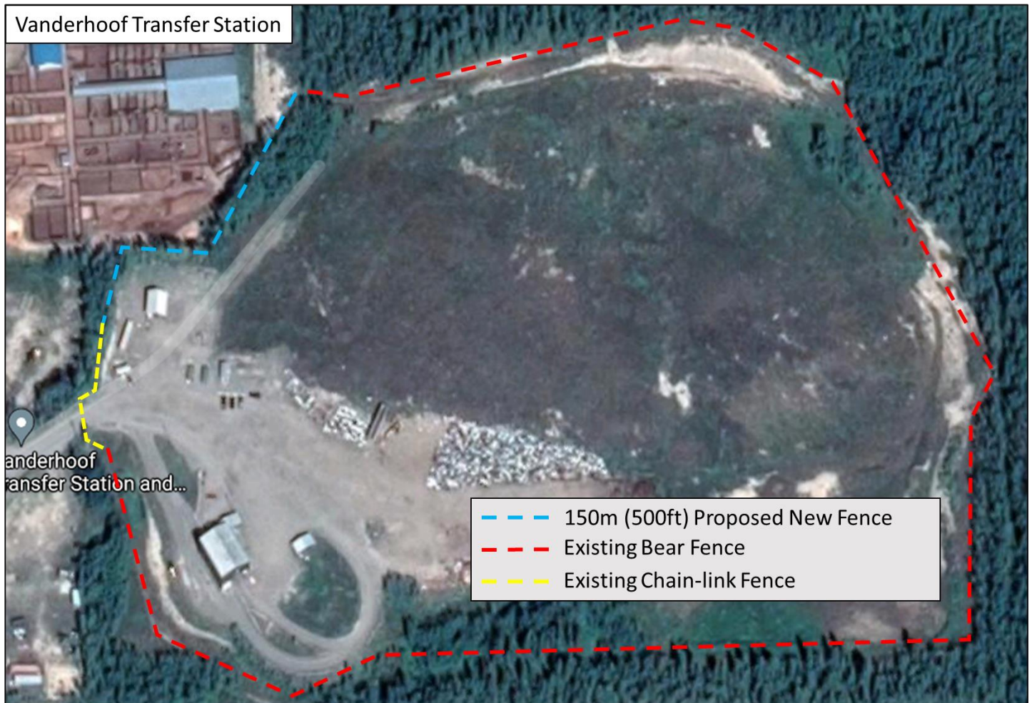
Figure 2. Fencing Plan
