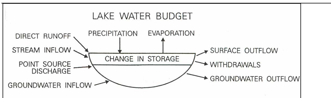
Figure 5: Schematic Water Budget (Holdren et al., 2001)
