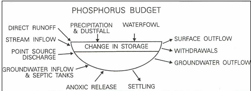
Figure 11: Schematic phosphorus budget (Holdren et al., 2001)
