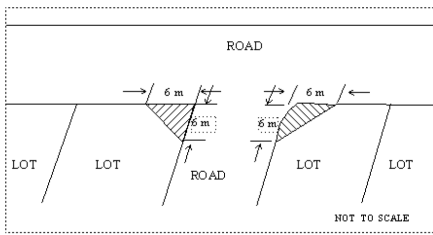
Diagram 1 – “Sight Triangle”
